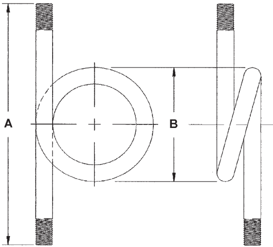
Type 910.15.100 Pigtail Siphon
