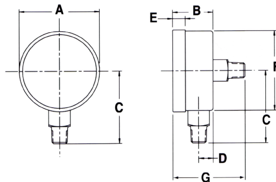
GAUGE DIMENSIONS
